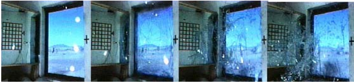
Unprotected annealed glass exposed to blast pressures (condition 5).
